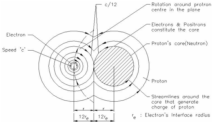
Fig. 11 Hydrogen Atom
