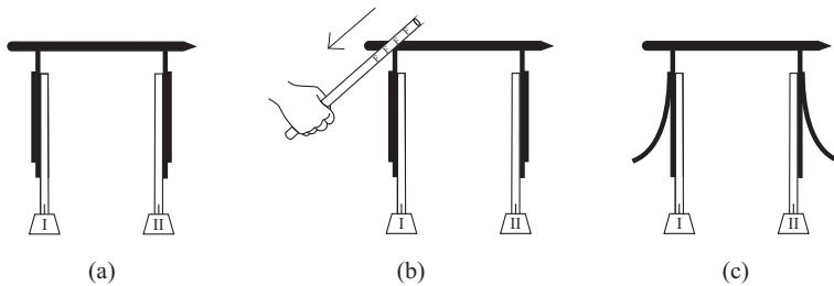
Figure 6.20: (a) Two initially discharged electroscopes connected by a wood skewer. (b) We scrape only electroscop I with an electrified straw. (c) The electrified straw is removed. We observe that both electroscopes have been charged.
