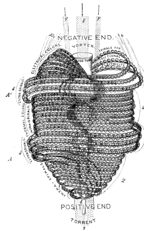
Fig 133. Piece of Atomic Spiral with 1st 2nd and 3rd Spirillæ.
