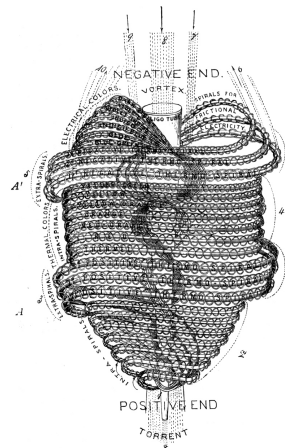
Fig 133. Piece of Atomic Spiral with 1st and 3rd Spirilla.
